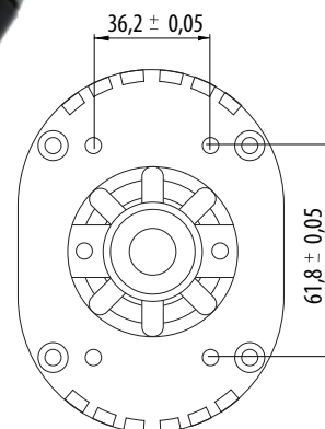
Fixing layout
