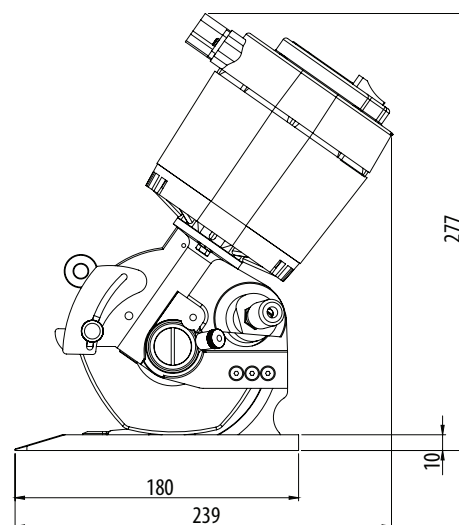
Dimension layout
